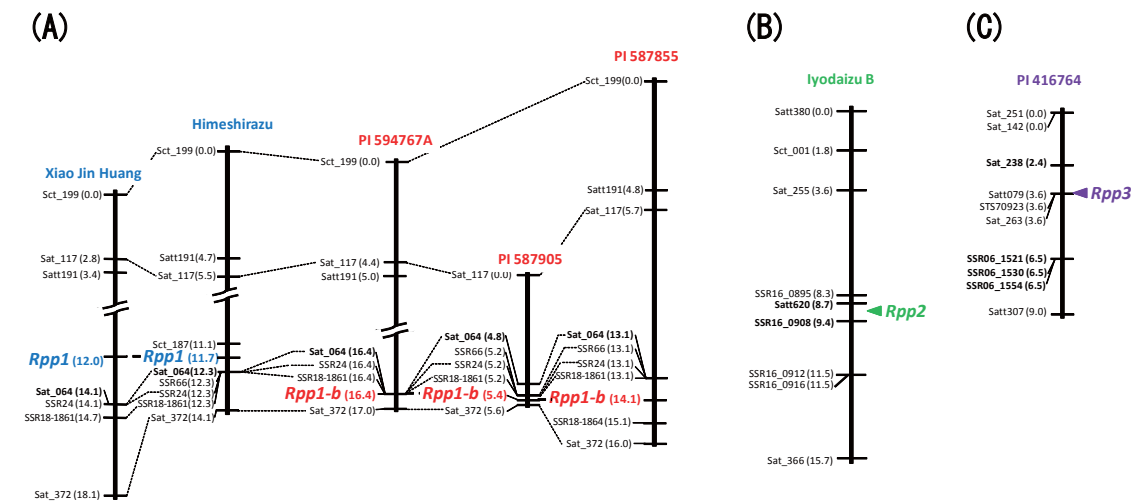
Fig. 1. Molecular linkage maps of ASR resistance loci in seven soybean varieties. It shows (A) soybean chromosome 18 where Rpp1 and Rpp1-b are located; (B) chromosome 16 where Rpp2 is located; and (C) chromosome 6 where Rpp3 is located. The loci Rpp2 and Rpp3 were determined by quantitative trait locus (QTL) analysis for sporulation level (SL) in ASR disease. The names of DNA markers and genetic distance (cM) from the top of linkage groups are shown on the left side of each linkage group.
