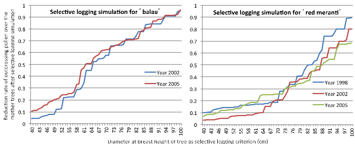
Fig. 2. Reduction rate of outcrossing pollen over the mother trees after selective logging simulation with every 1cm increment of cutting limit from 40 to 100cm (below)
