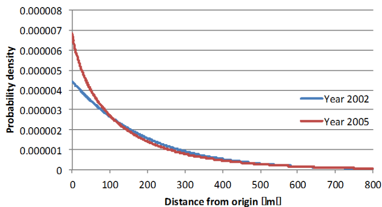
Fig. 1. Pollen dispersal pattern of Shorea maxwelliana recognized as 'balau' in two flowering events with different flowering magnitude (left).
