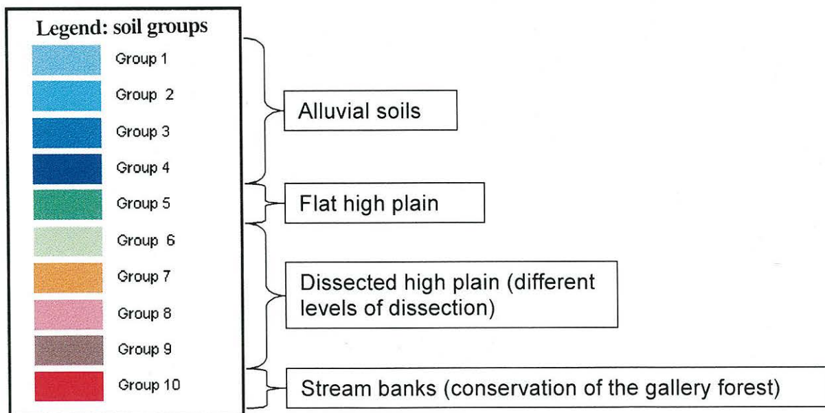
Fig. 2 Land suitability soil groups defined from a 1:100,000 soil map (IGAC, 1978). Soil limiting factors and suitable land uses for these groups are given in Table 1, in function of the position within the landscape
