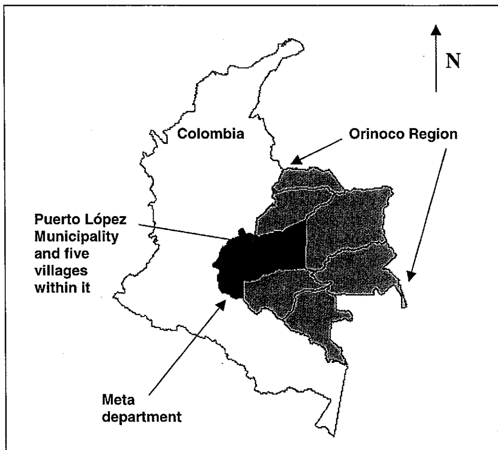
Fig. 1 Nested test sites in the Colombian Orinoco region, within Colombia
