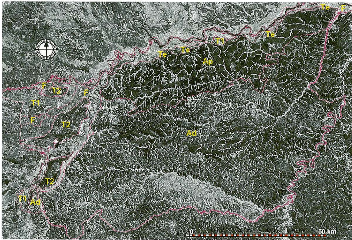
Fig. 3 General map of landscape types overlaid on a portion of a mosaic of JERS-1 images acquired in 1995 ((c)NASDA, 1998), over the municipality of Puerto López. Landscape types presented are the flat high plains (Ap), the dissected high plains (Ad), depositional alluvial terraces (T1 and T2), floodplains (F) and erosional terraces (Te)
