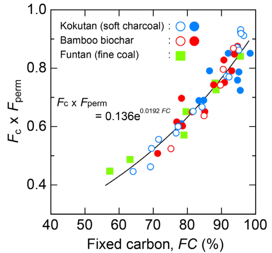
Figure 3.3. Relationship between FC and the product of F_c and F_{perm} . F_{perm} is calculated at a soil temperature of 14.9 °C (Adapted from Kurimoto et al. 2024).
