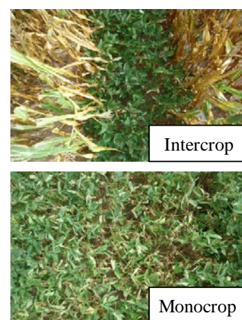
Fig. 2. Comparison of soybean growth after a long dry spell in Nampula.
