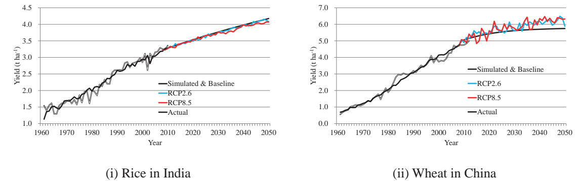
Fig. 2. Trends in crop yield
