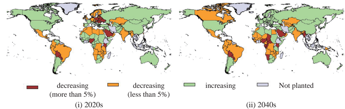
Fig. 3. Effects of climate change on wheat yield: differences between baseline and RCP6.0
