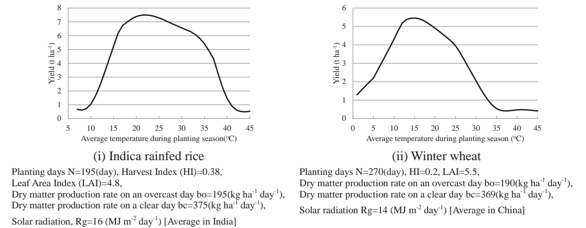
Fig. 1. Relationship between potential yield and temperature
