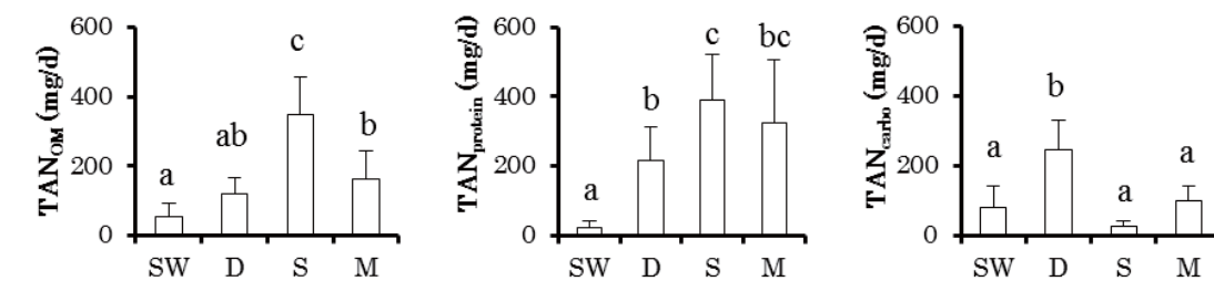
Fig. 2. Daily total assimilated nutrients (TAN) in juvenile H. scabra as obtained as the product of ADC and daily feed ingestion rate; assimilated organic matter ( TAN_{\text{OM}} ), crude protein ( TAN_{\text{protein}} ) and crude carbohydrate ( TAN_{\text{carbo}} ). The mean body weight of H. scabra was 10 g. Different letters (i.e. a, b and c) indicate statistically significant difference ( p < 0.05 ).
