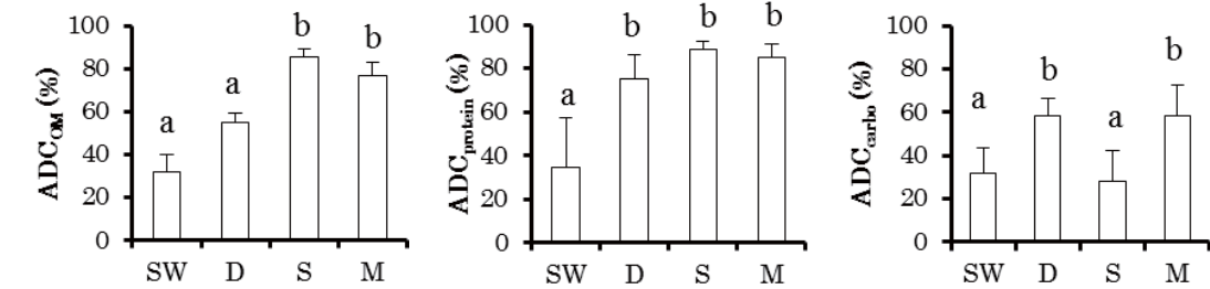
Fig. 1. Apparent digestibility coefficient of organic matter ( ADC_{\text{OM}} ), crude protein ( ADC_{\text{protein}} ) and crude carbohydrate ( ADC_{\text{carbo}} ) of seaweed (SW), diatom (D), shrimp meal (S) and mussel meal (M) in juvenile Holothuria scabra . ADC was obtained from the difference in nutrient contents between diet and feces. Different letters (i.e. a and b) indicate statistically significant difference ( p < 0.05 ).
